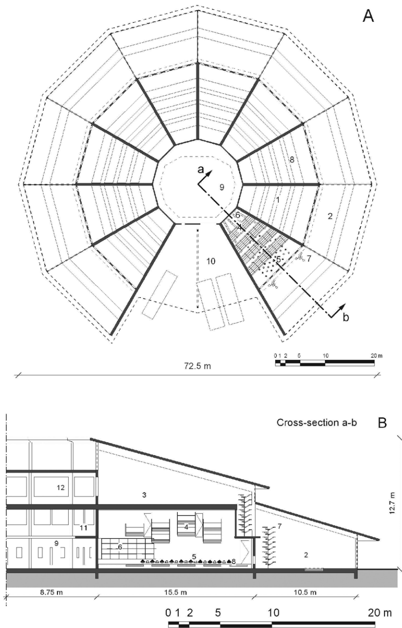
Figure 5. Roundel design. Top view (A) and cross-section a-b of one segment (B). 1: unit for 3000 hens; 2 & 3: foraging areas; 4: perches (for resting) over manure belts; 5: water and feed supply; 6: laying nests; 7: artificial trees; 8: manure belts at floor level; 9: room for collecting eggs; 10: expedition; 11: visitors and control gallery; 12: technical installations. (drawn by JvR Architectuur)
